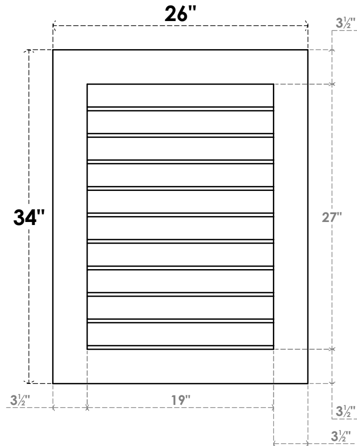
FRONT
