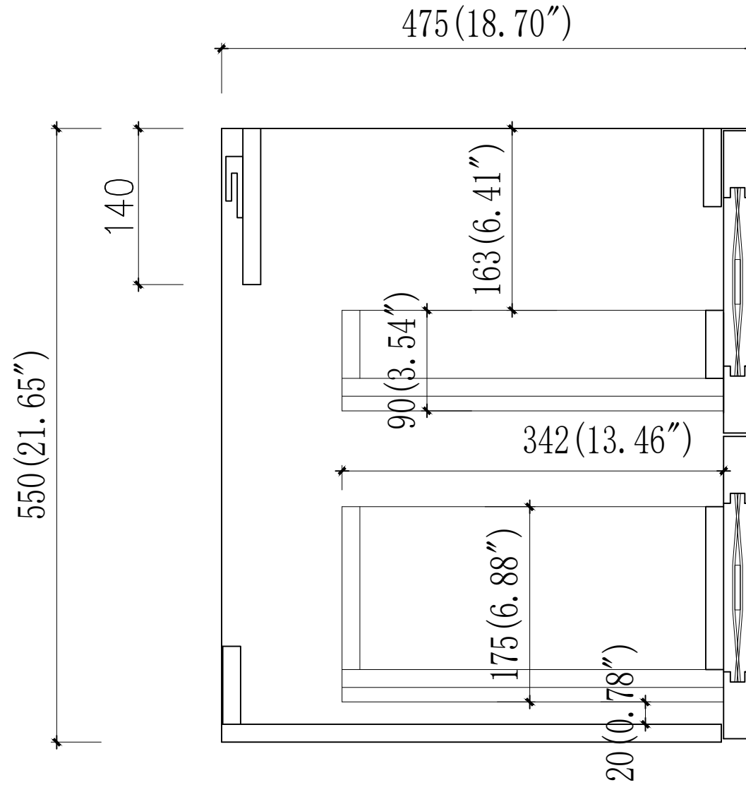
Drawer Detail
