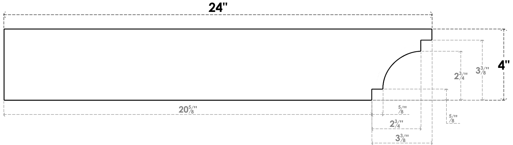
SIDE PROFILE
