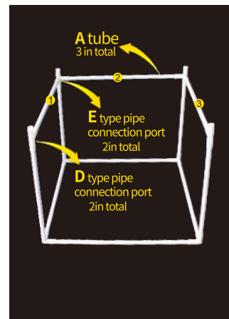
③. Insert the 2 E-shaped pipe connection ports and the 2 D-shaped pipe connection ports on the B pipe, and then connect the A pipe, as shown in the figure above
