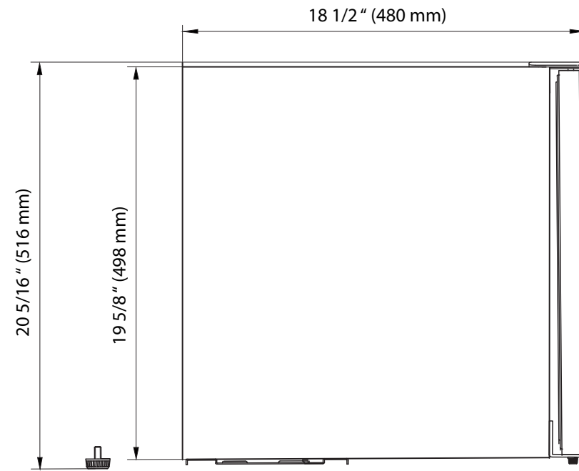
Side View
