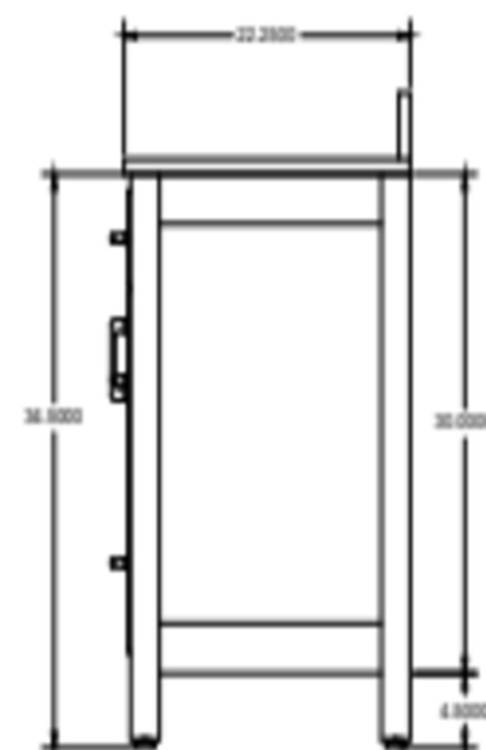
SIDE VIEW
