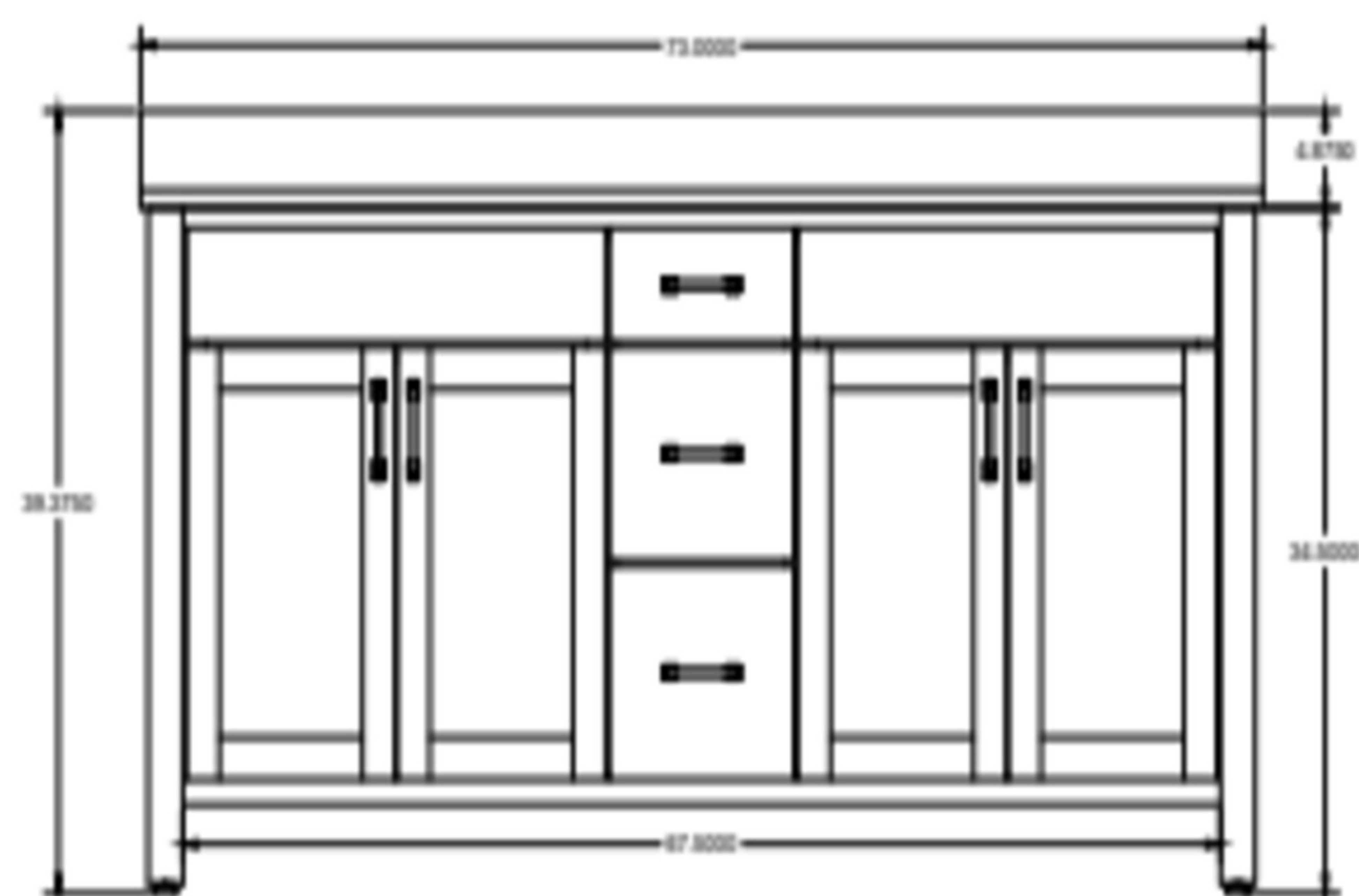
FRONT VIEW
