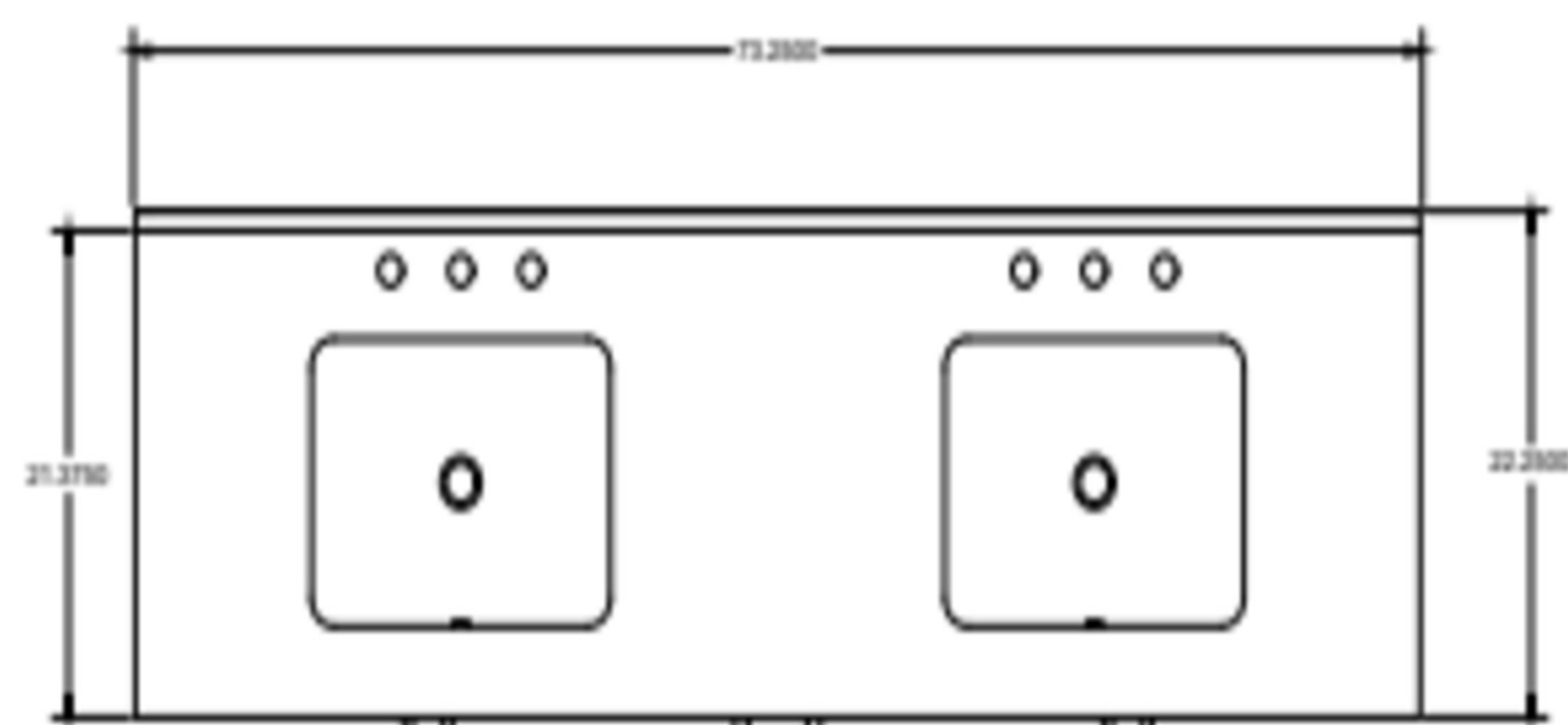
TOP VIEW
