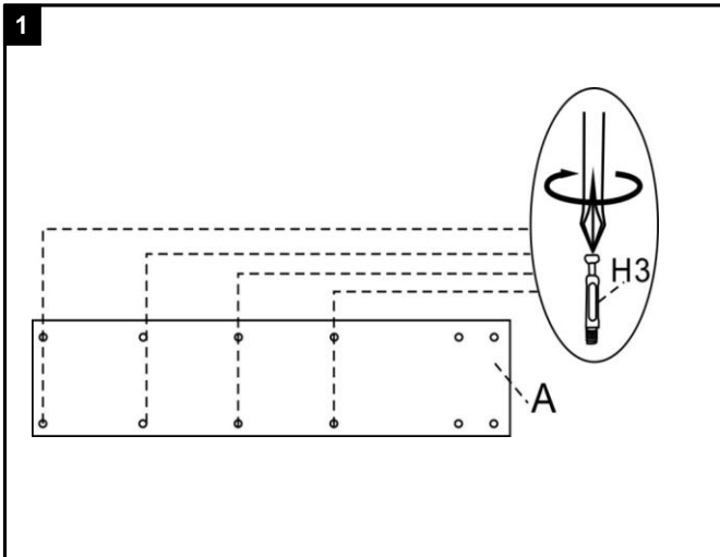
Step 1 Attach the Screw(H3) to Side panel(A) Tighten with philps driver
