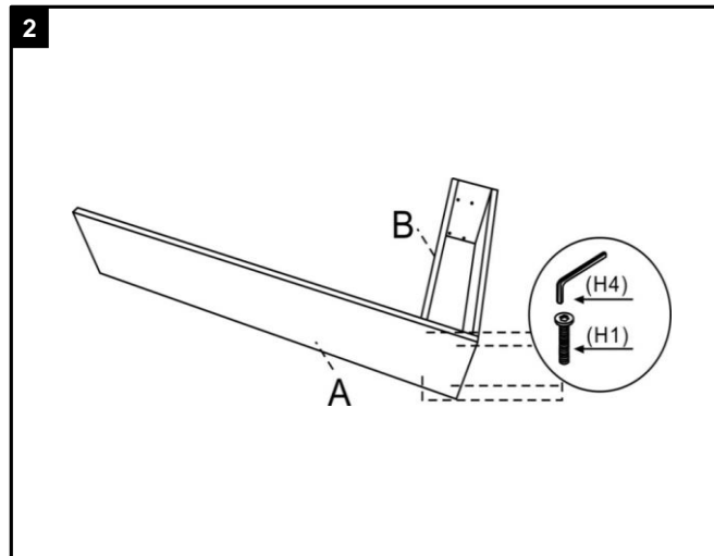
Step 2 Attach the Box(B) to Side panel(A), using Allen bolt(H1) Tighten with Allen key(H4)
