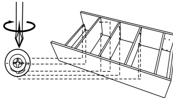
Step 6 Attach the Top panel(D)and Shelf(C)to Side panel(A) Tighten with philips driver
