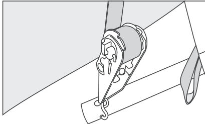
Figure L: Inserting Hook into Corner Leg
