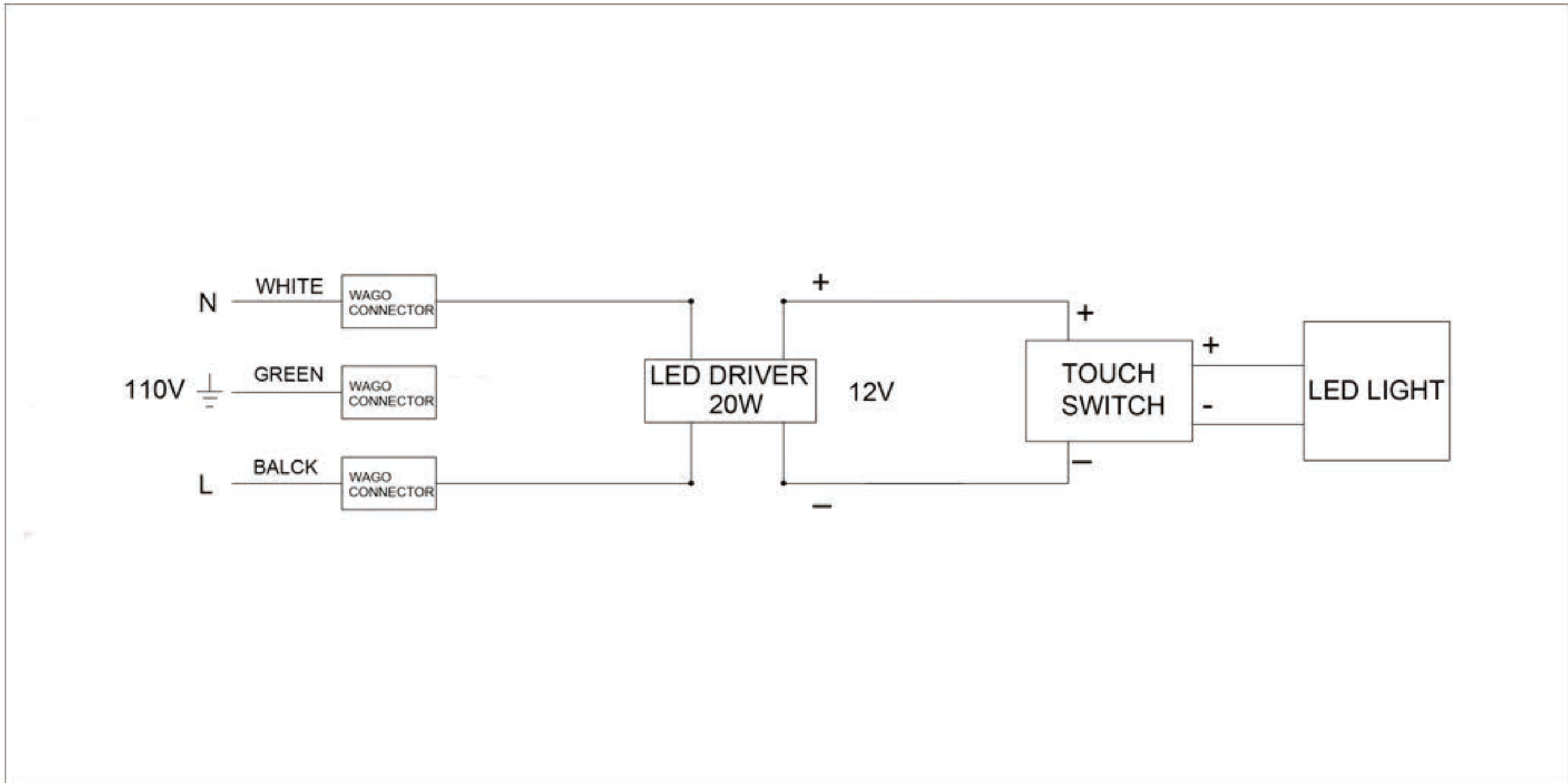
Circuit Diagram
