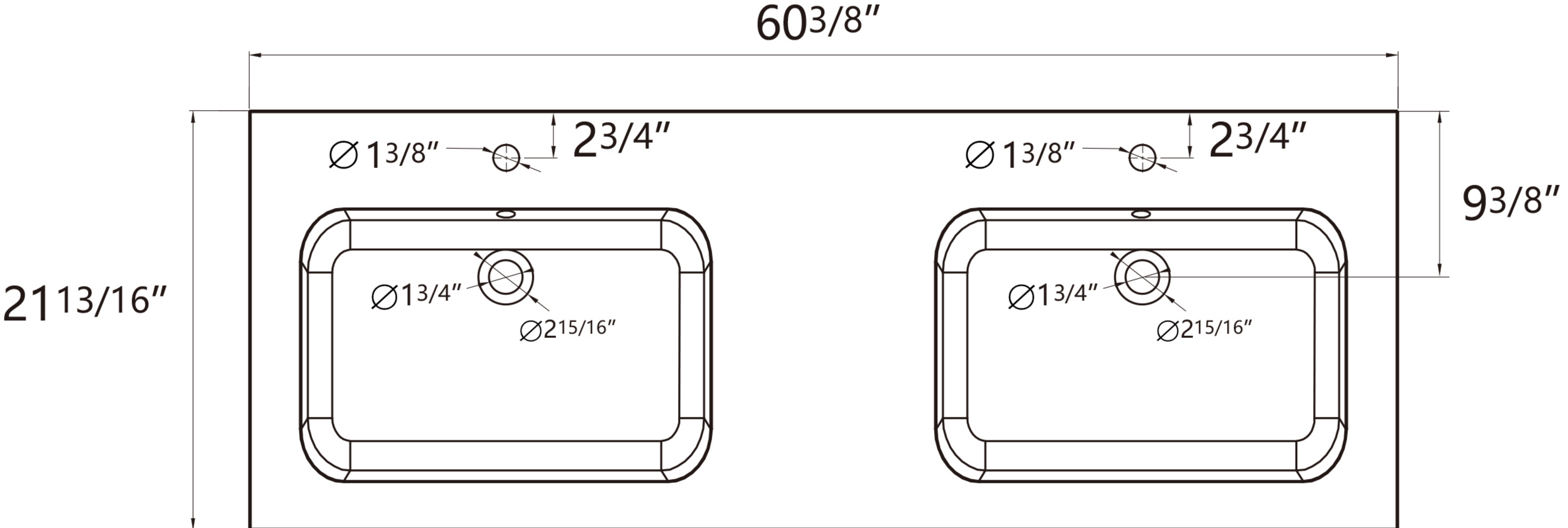
Top View
