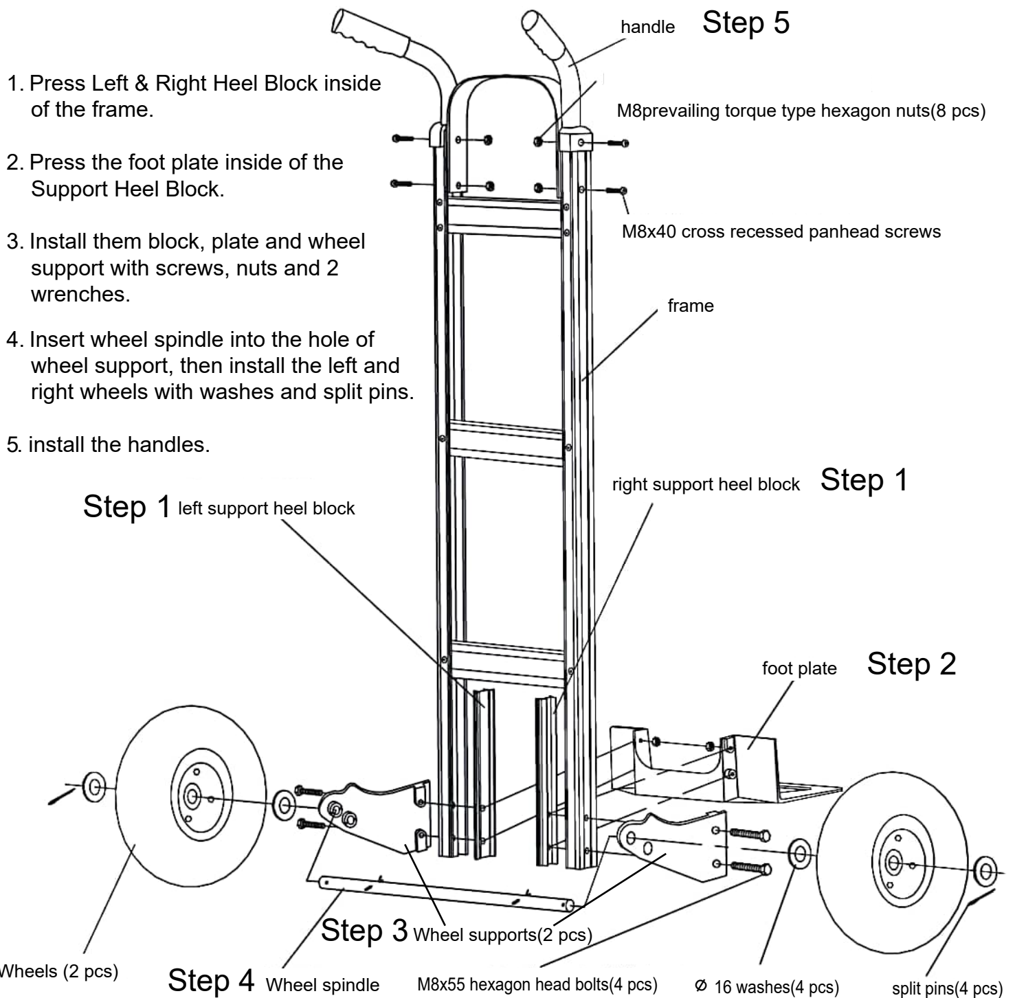
2125A Assembly diagram
