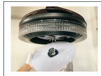
Step 6. Connect the Bluetooth drive cable on the PVC panel to the Bluetooth cable on the chassis of the fan lamp host, and put the PVC panel into the lamp shade at the same time.
