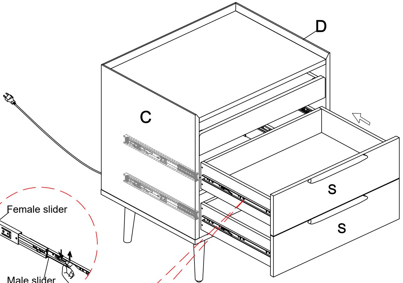
Schematic diagram of slide rail disassembly
