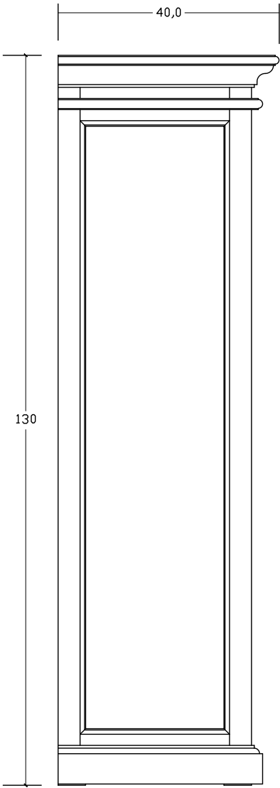
SIDE VIEW
