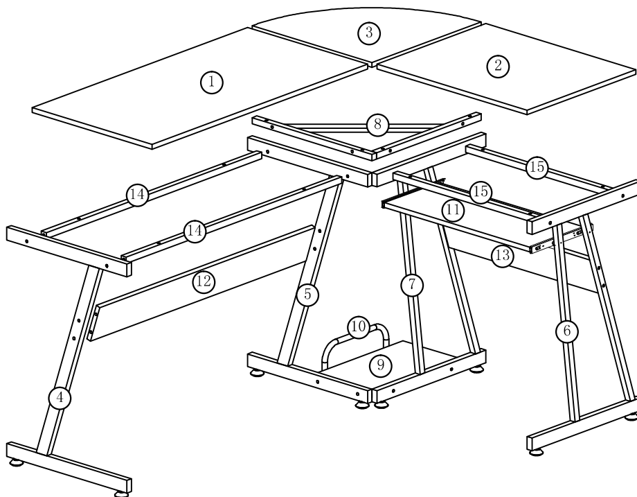
Decomposition Diagram
