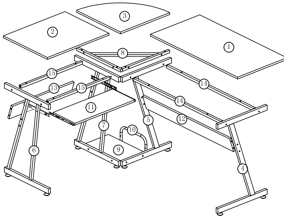
Decomposition Diagram
