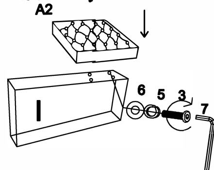
STEP-2 How to assembly arm
