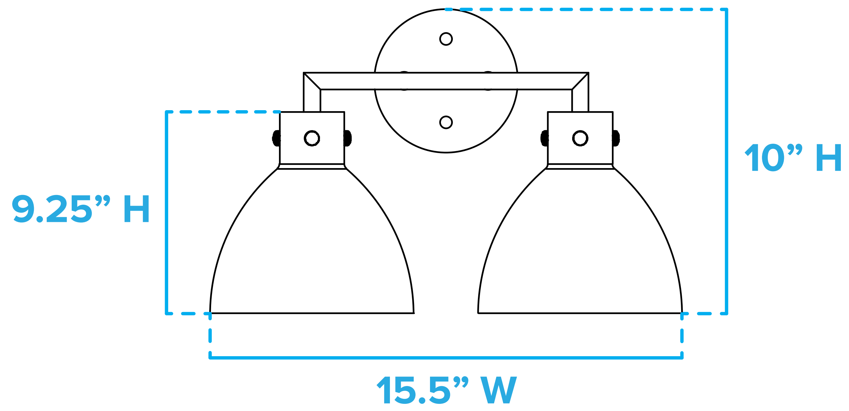
Front View
