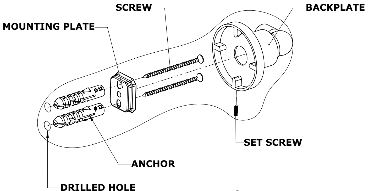
DETAIL O
