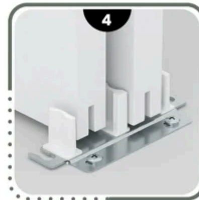
Install floor guide
